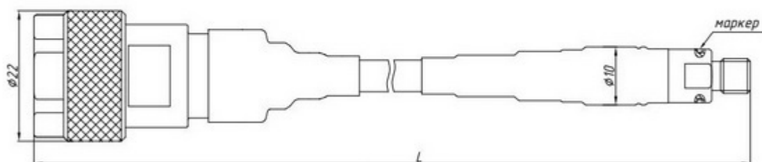
KC18A-01-13P
