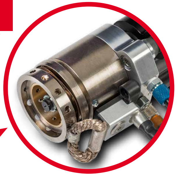
PH-9 SRM 12 +G Integrierter Massekontakt Integrated ground contact
