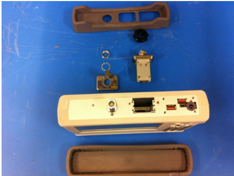
Figure 4-7. Both Bumpers, Batteries, Battery Cover, RF Out Mounting Plate and InstaCal/PM Module Removed
