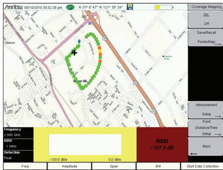
Coverage Mapping outdoors
