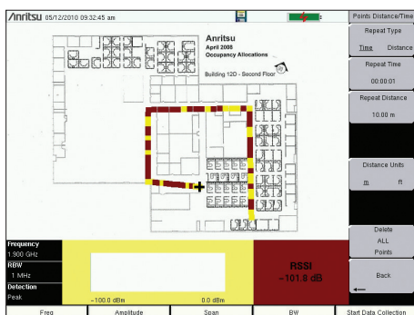
Coverage Mapping indoors
