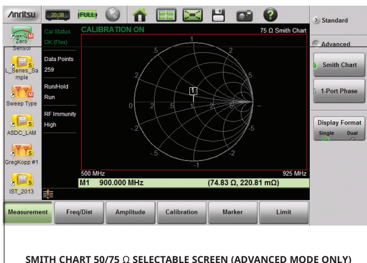
SMITH CHART 50/75 Ω SELECTABLE SCREEN (ADVANCED MODE ONLY)
