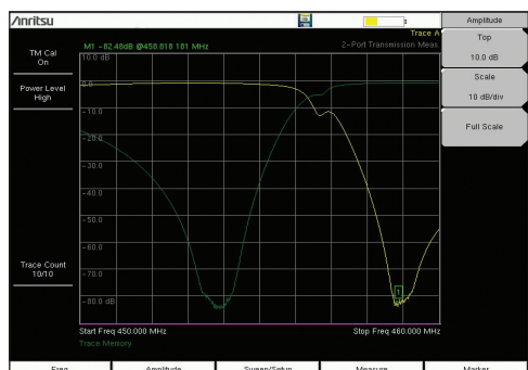
Duplexer Measurement
