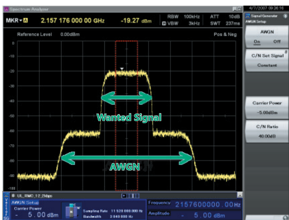
Wanted Signal + AWGN Signal output from one unit
